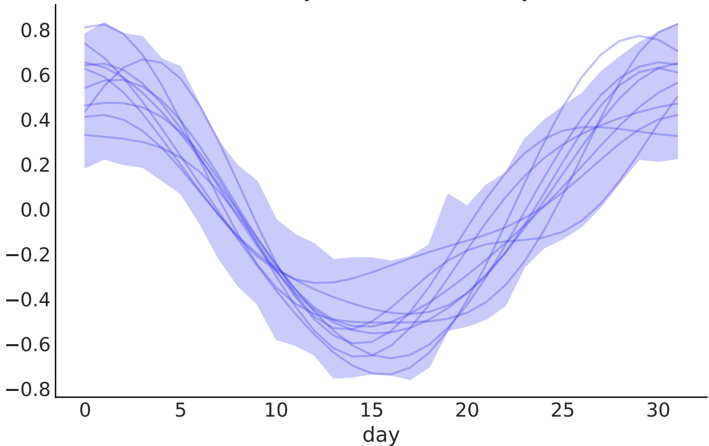
Monthly Fourier Seasonality
