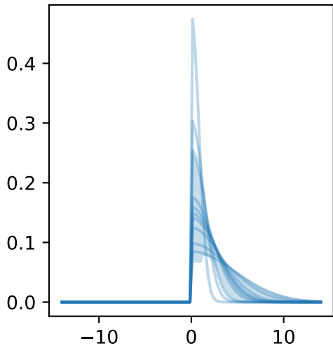
event=PyData-Berlin
